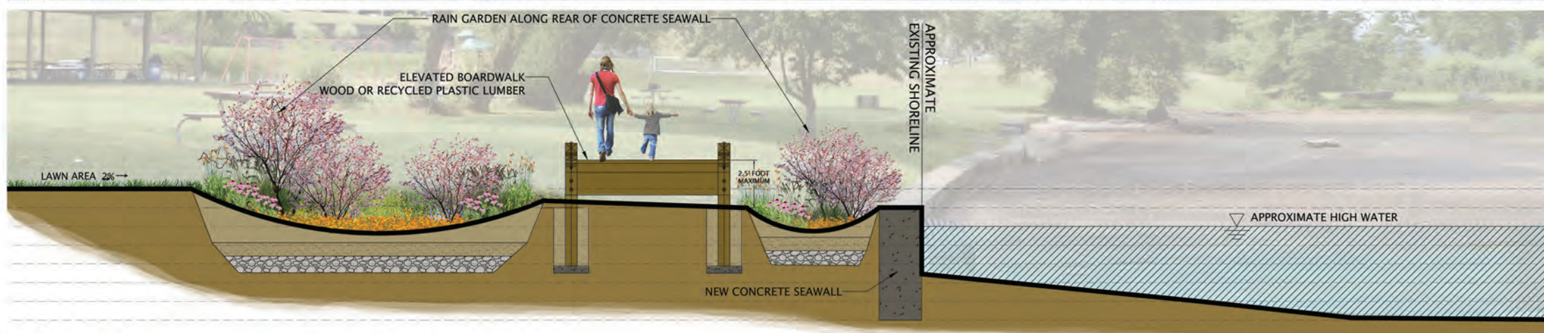
1 TYPICAL BOARDWALK AND RAIN GARDENS CLA-1 SCALE: N.T.S
