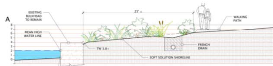
Section A of 2022 'Freer Park Bulkhead & Green Infrastructure improvements'
